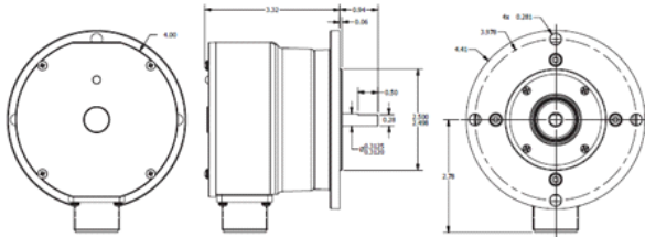
5/16" SHAFT WITH FLAT | PY FLANGE | 10 PIN MS CONNECTOR
